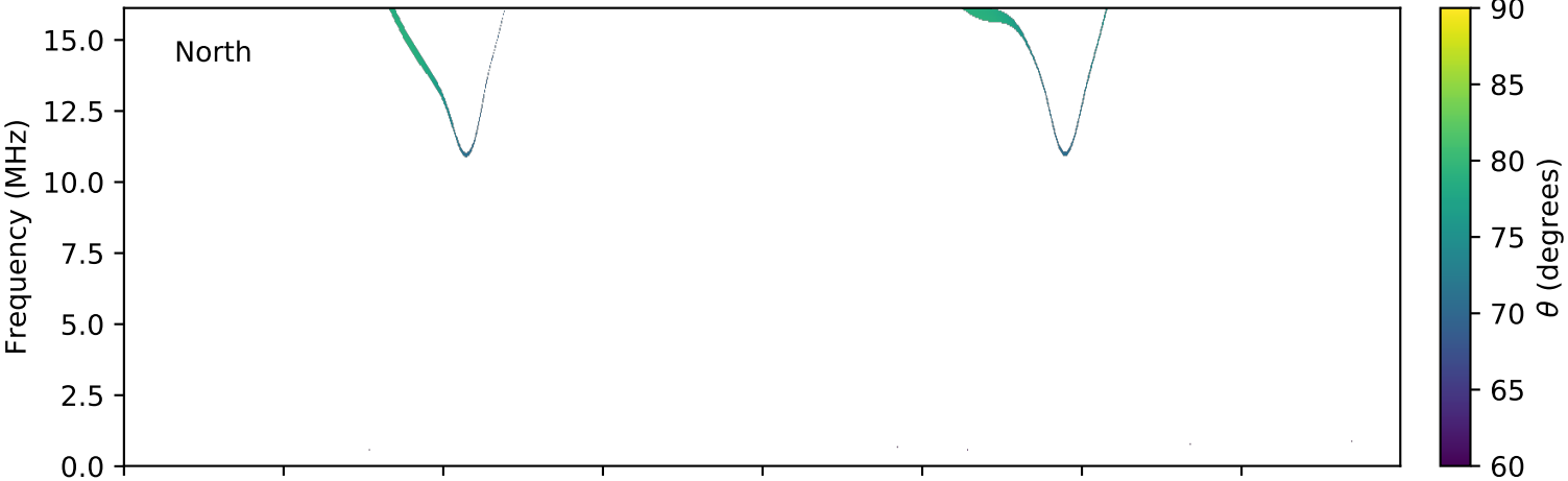
expres_cassini_jupiter_europa_isaac_lossc-wid1deg_3kev_20020623_v01.cdf
