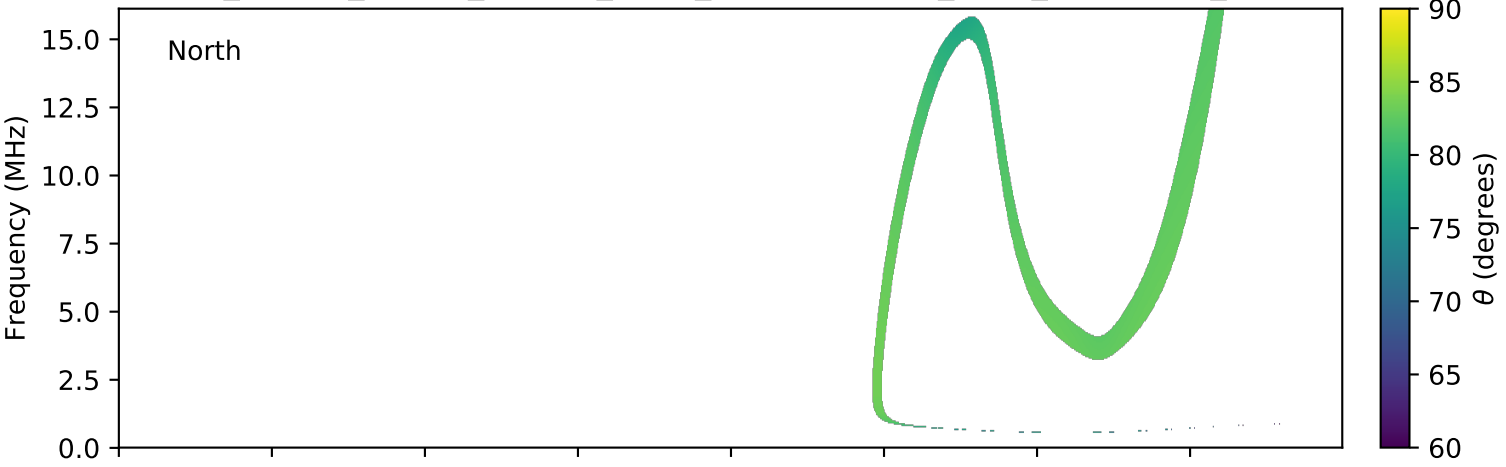
expres_cassini_jupiter_europa_isaac_lossc-wid1deg_3kev_20020622_v01.cdf
