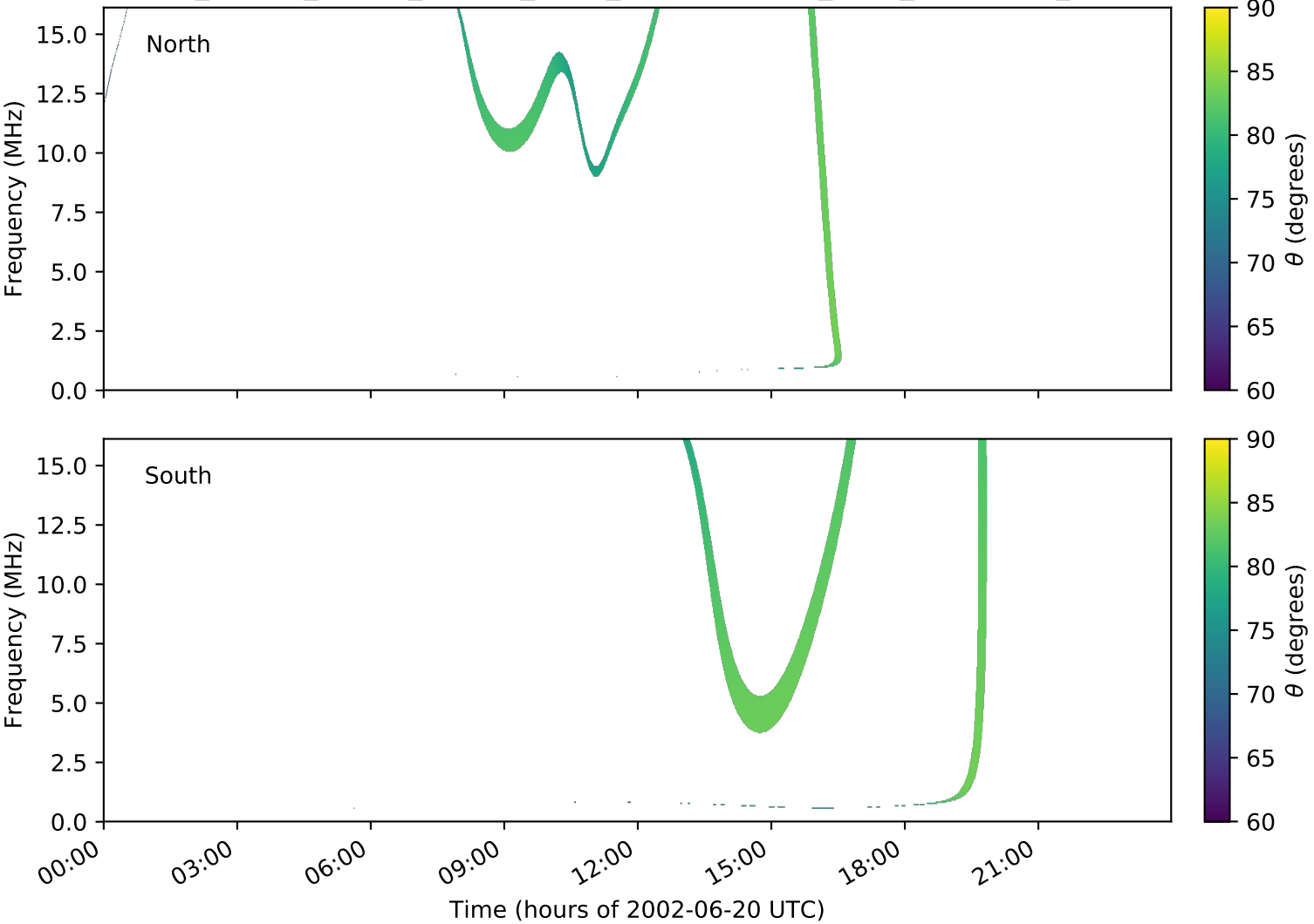
expres_cassini_jupiter_europa_isaac_lossc-wid1deg_3kev_20020620_v01.cdf
