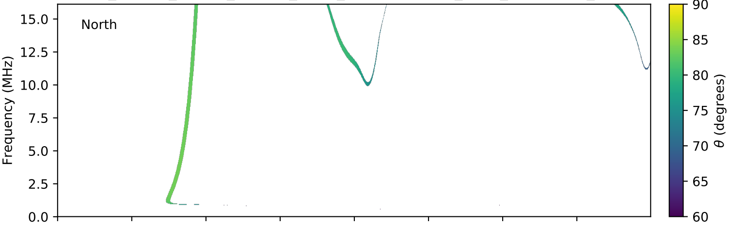
expres_cassini_jupiter_europa_isaac_lossc-wid1deg_3kev_20020619_v01.cdf
