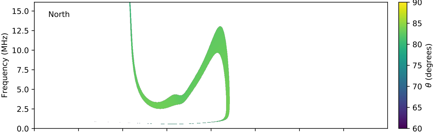
expres_cassini_jupiter_europa_isaac_lossc-wid1deg_3kev_20020606_v01.cdf
