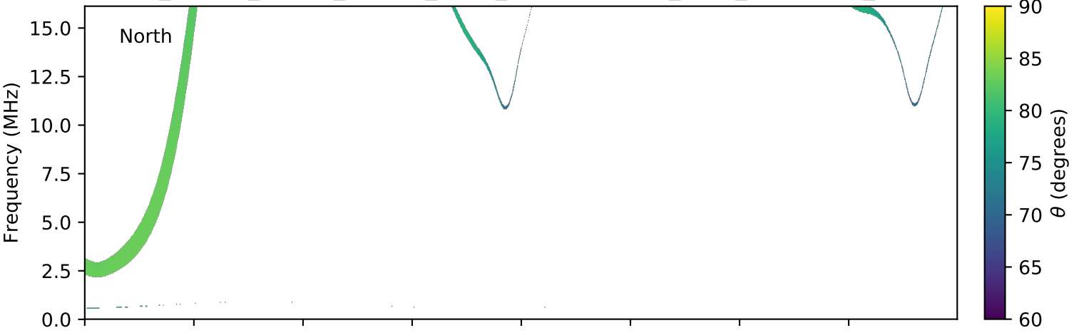
expres_cassini_jupiter_europa_isaac_lossc-wid1deg_3kev_20020605_v01.cdf
