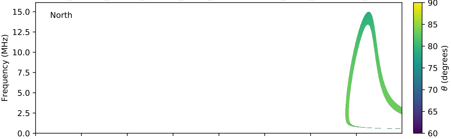
expres_cassini_jupiter_europa_isaac_lossc-wid1deg_3kev_20020604_v01.cdf
