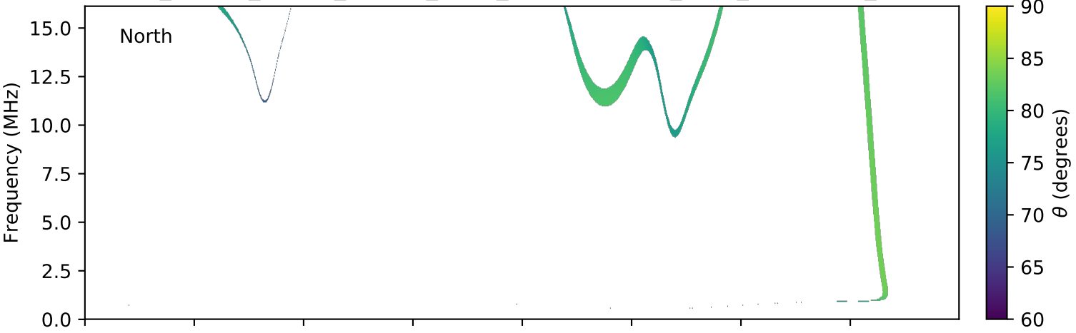
expres_cassini_jupiter_europa_isaac_lossc-wid1deg_3kev_20020602_v01.cdf
