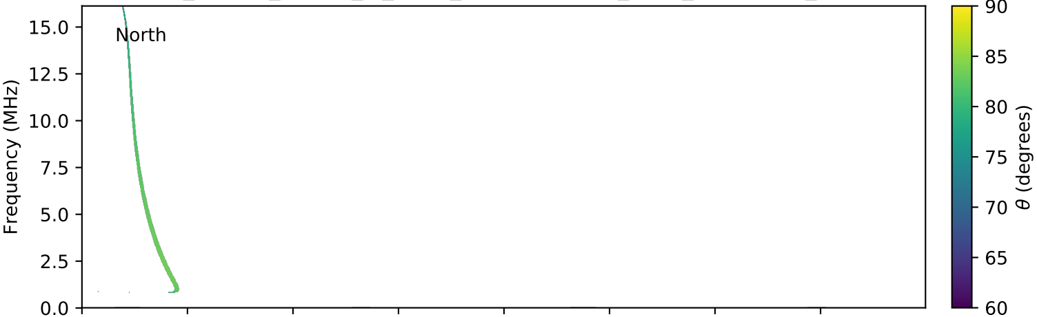
expres_cassini_jupiter_io_isaac_lossc-wid1deg_3kev_20011229_v01.cdf
