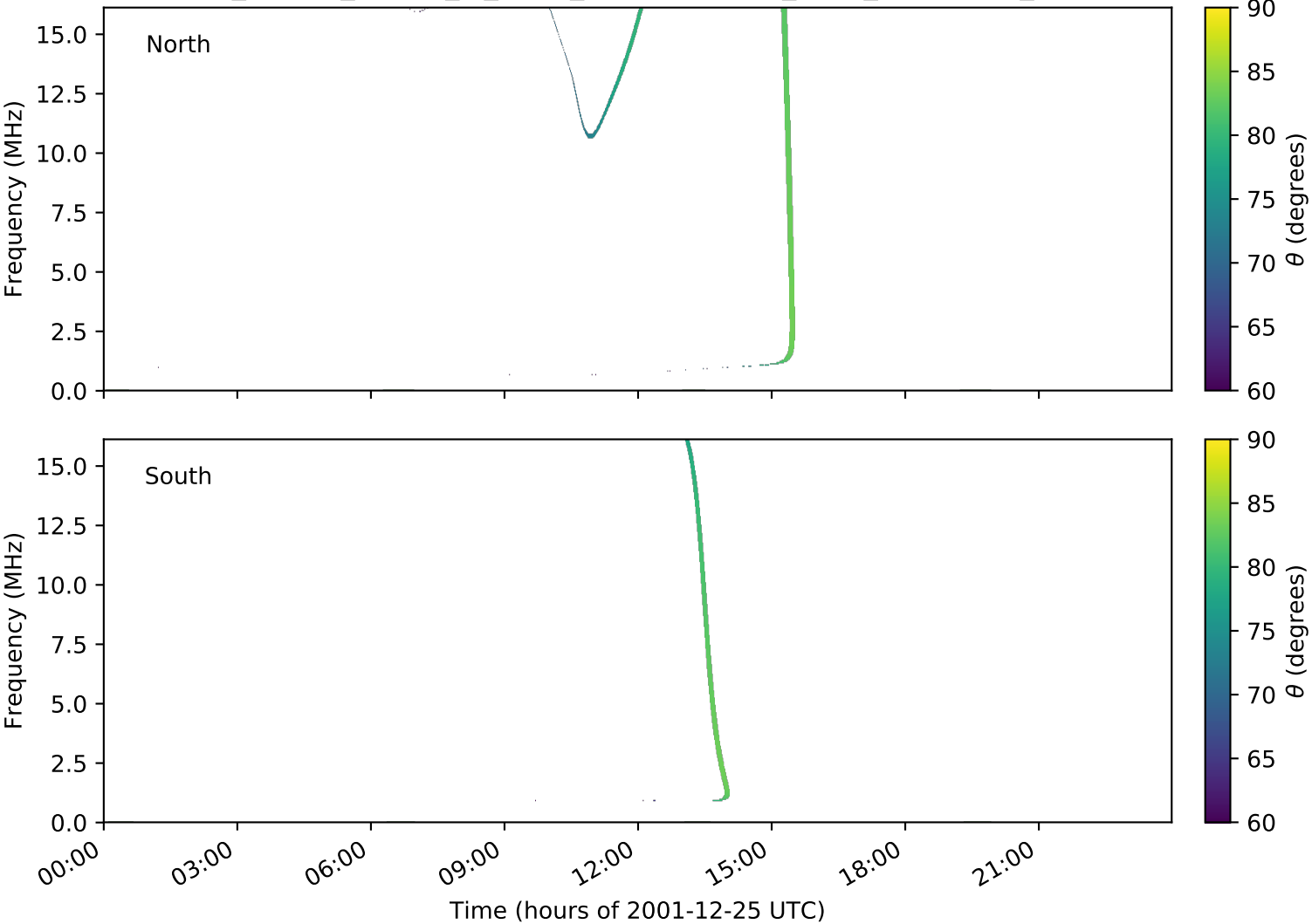
expres_cassini_jupiter_io_isaac_lossc-wid1deg_3kev_20011225_v01.cdf
