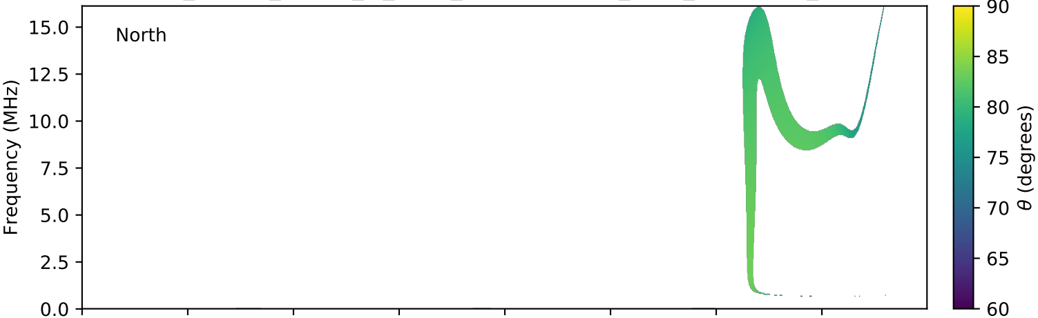
expres_cassini_jupiter_io_isaac_lossc-wid1deg_3kev_20011224_v01.cdf
