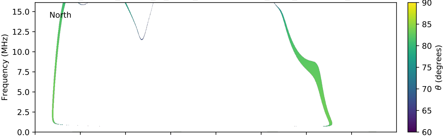
expres_cassini_jupiter_io_isaac_lossc-wid1deg_3kev_20011223_v01.cdf
