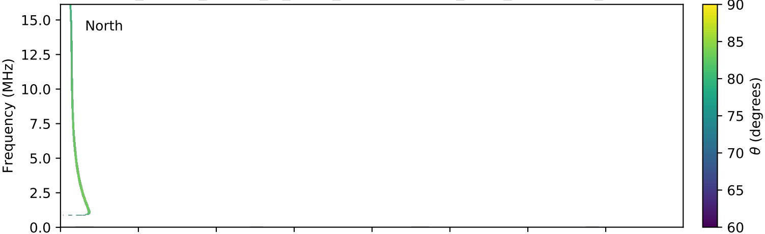
expres_cassini_jupiter_io_isaac_lossc-wid1deg_3kev_20011222_v01.cdf
