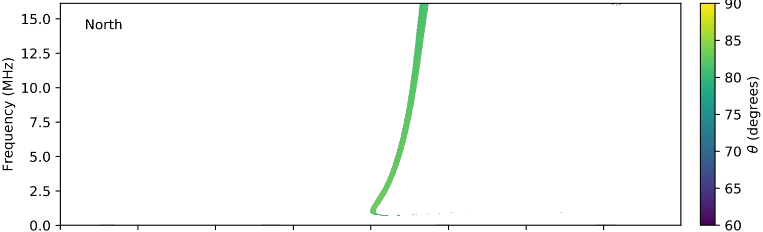
expres_cassini_jupiter_io_isaac_lossc-wid1deg_3kev_20011219_v01.cdf
