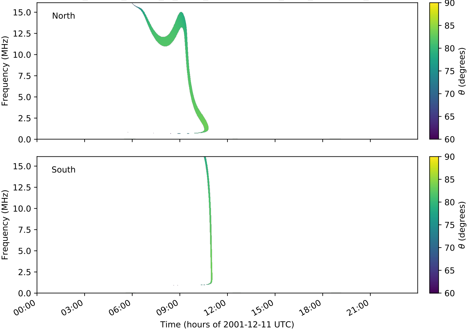
expres_cassini_jupiter_io_isaac_lossc-wid1deg_3kev_20011211_v01.cdf
