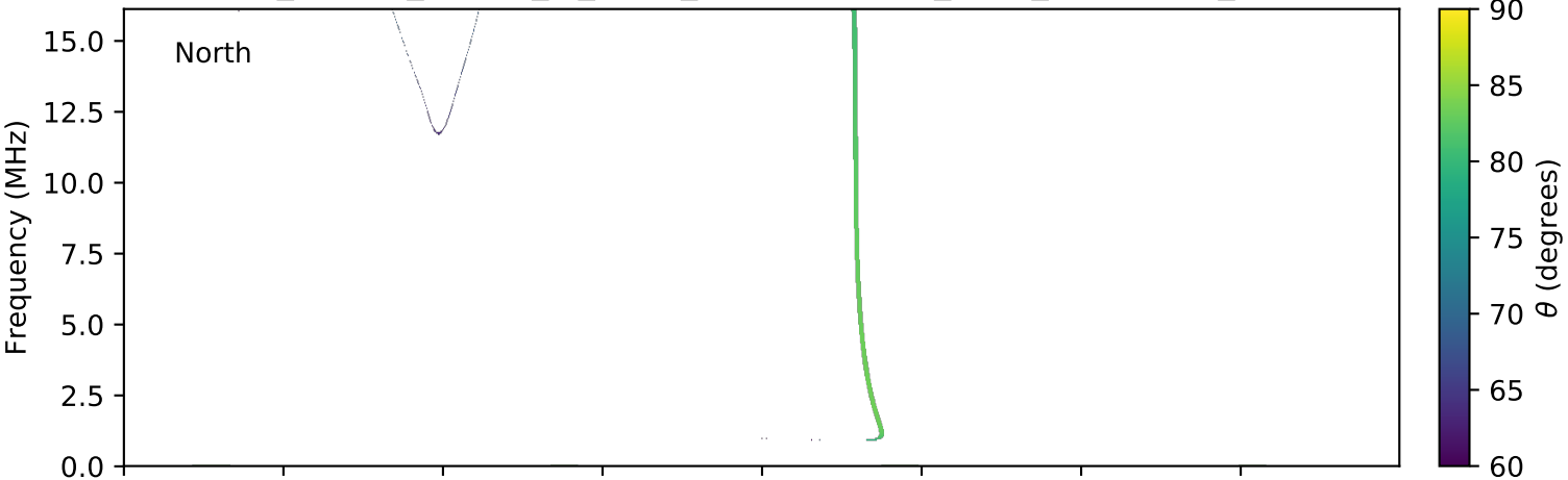
expres_cassini_jupiter_io_isaac_lossc-wid1deg_3kev_20011202_v01.cdf
