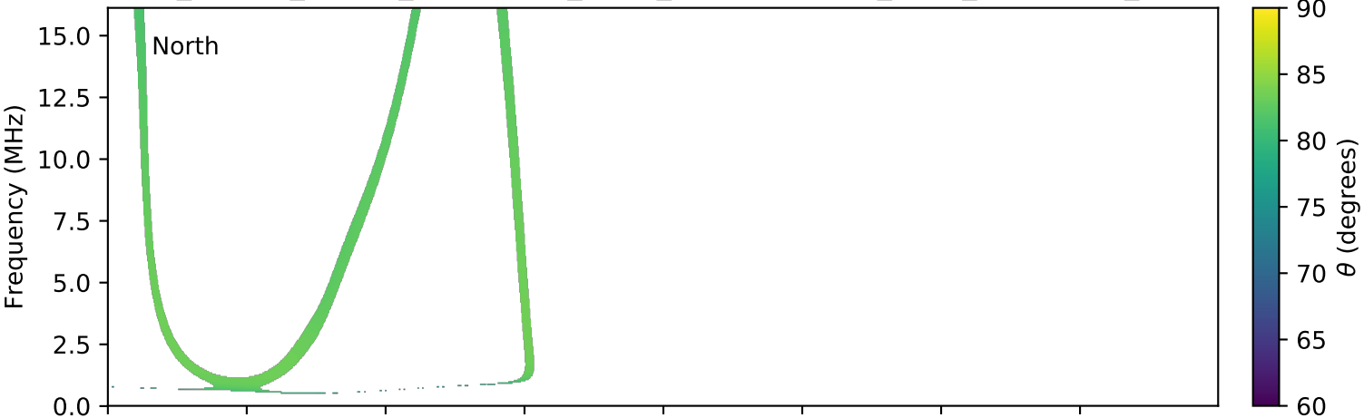
expres_cassini_jupiter_ganymede_isaac_lossc-wid1deg_3kev_20011229_v01.cdf
