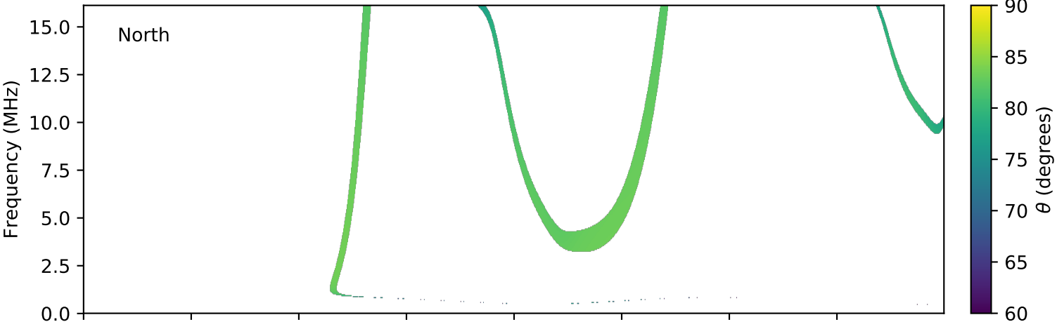
expres_cassini_jupiter_ganymede_isaac_lossc-wid1deg_3kev_20011226_v01.cdf
