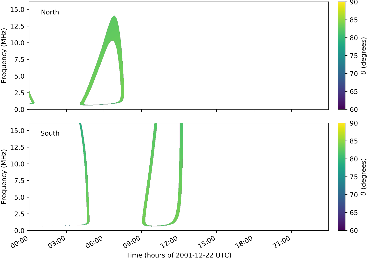
expres_cassini_jupiter_ganymede_isaac_lossc-wid1deg_3kev_20011222_v01.cdf
