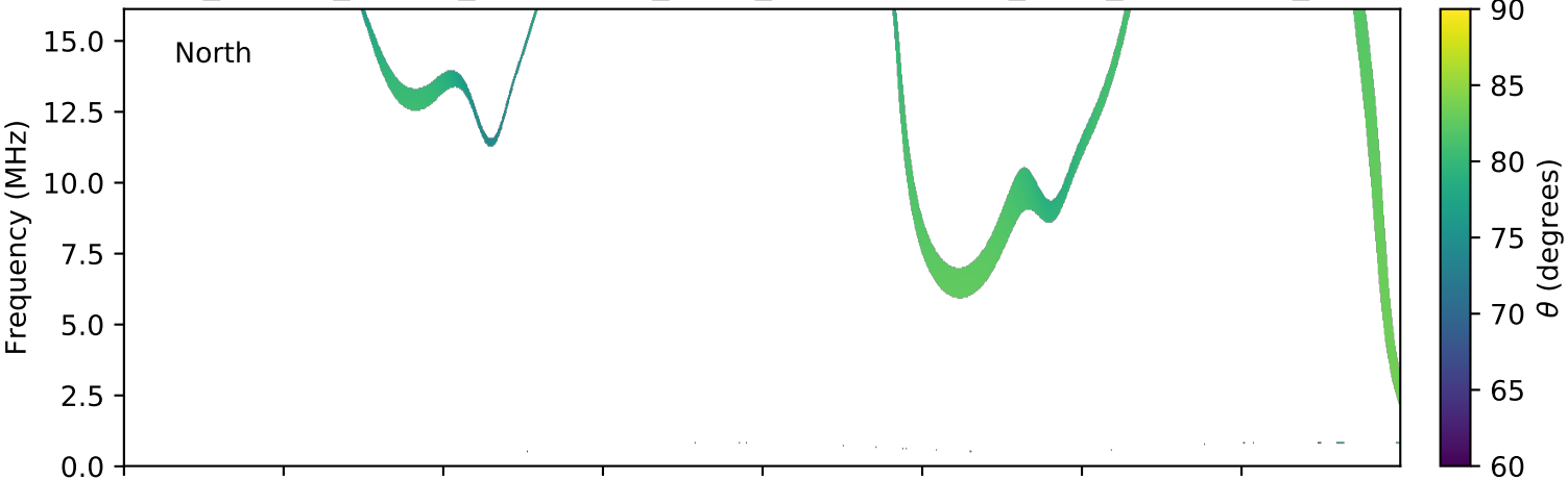
expres_cassini_jupiter_ganymede_isaac_lossc-wid1deg_3kev_20011221_v01.cdf
