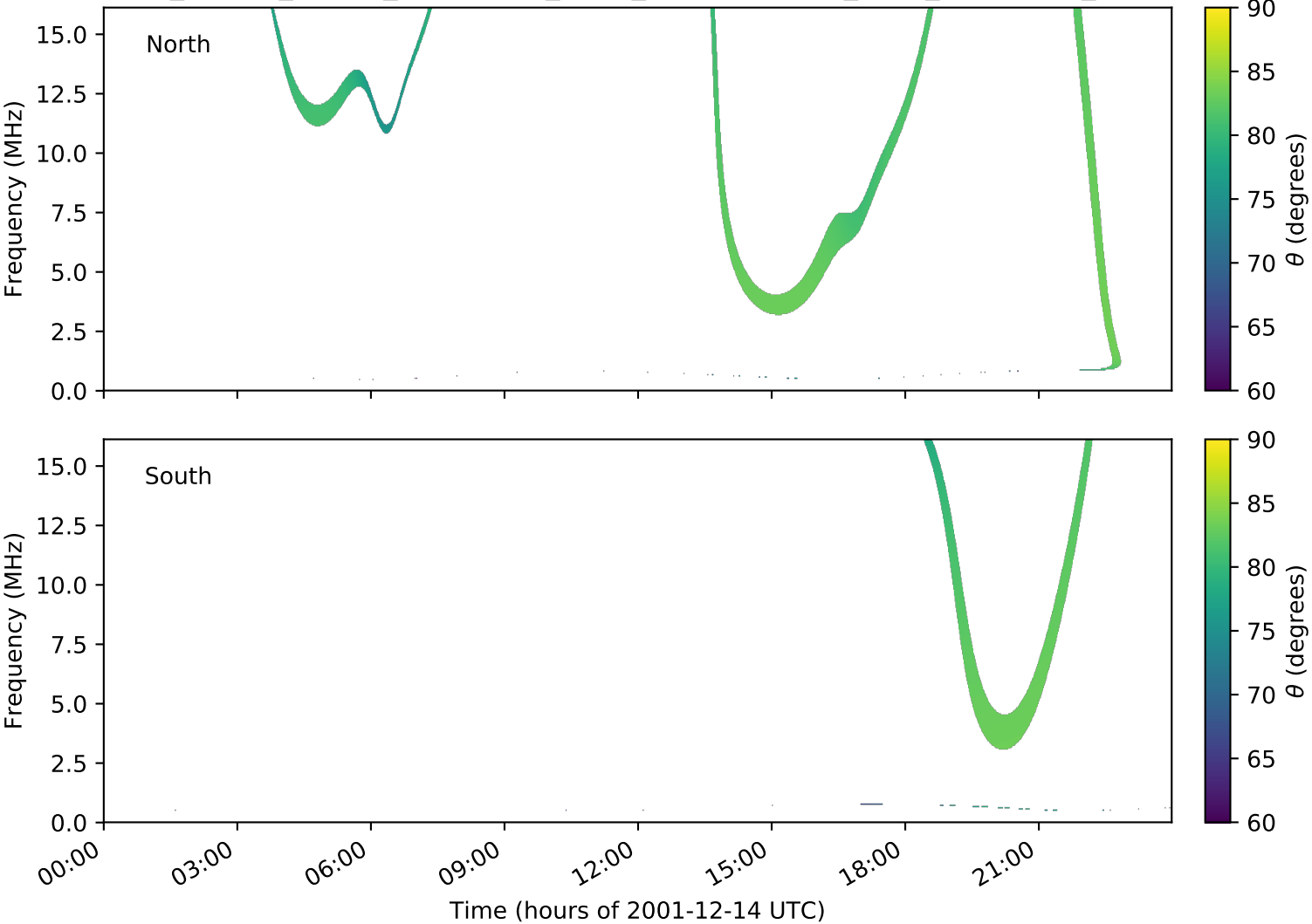
expres_cassini_jupiter_ganymede_isaac_lossc-wid1deg_3kev_20011214_v01.cdf
