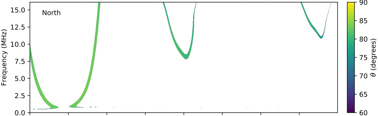
expres_cassini_jupiter_ganymede_isaac_lossc-wid1deg_3kev_20011212_v01.cdf
