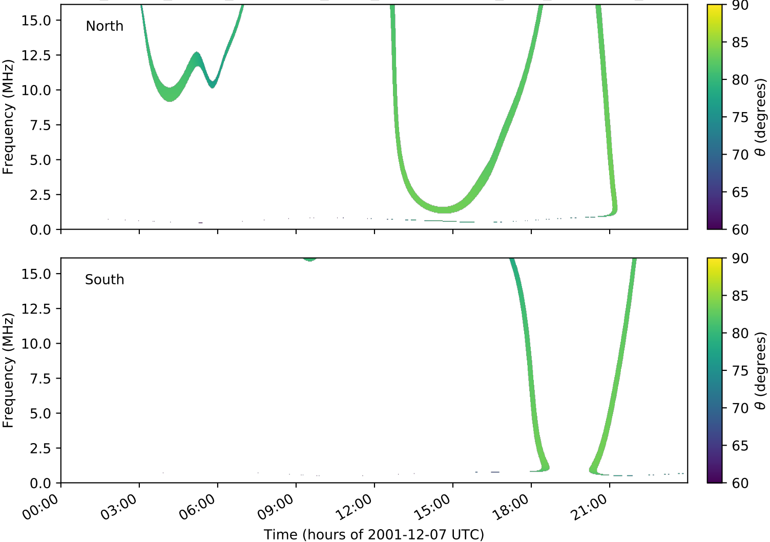
expres_cassini_jupiter_ganymede_isaac_lossc-wid1deg_3kev_20011207_v01.cdf
