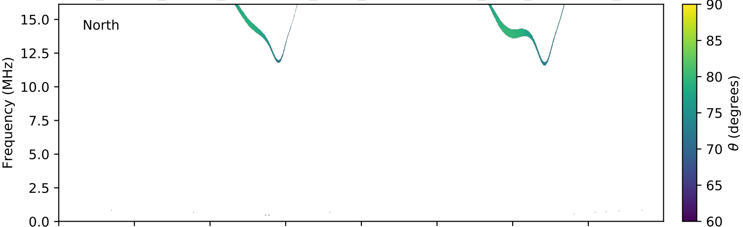
expres_cassini_jupiter_ganymede_isaac_lossc-wid1deg_3kev_20011206_v01.cdf
