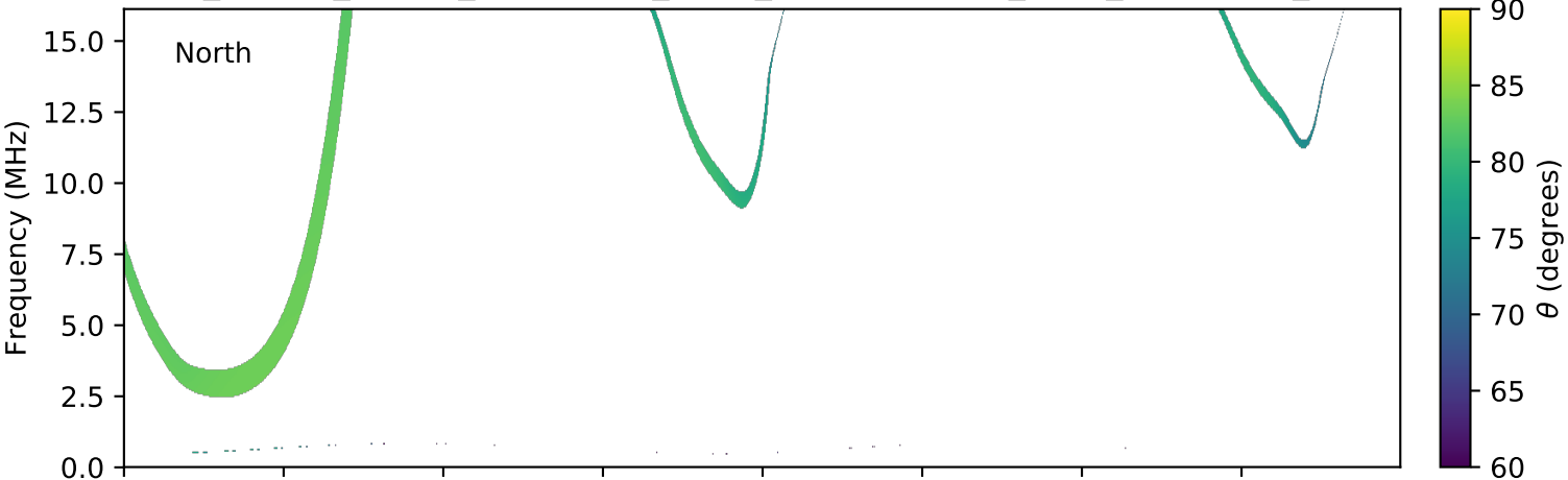
expres_cassini_jupiter_ganymede_isaac_lossc-wid1deg_3kev_20011205_v01.cdf
