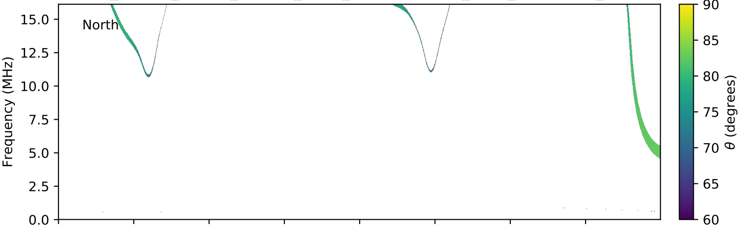
expres_cassini_jupiter_europa_isaac_lossc-wid1deg_3kev_20011231_v01.cdf
