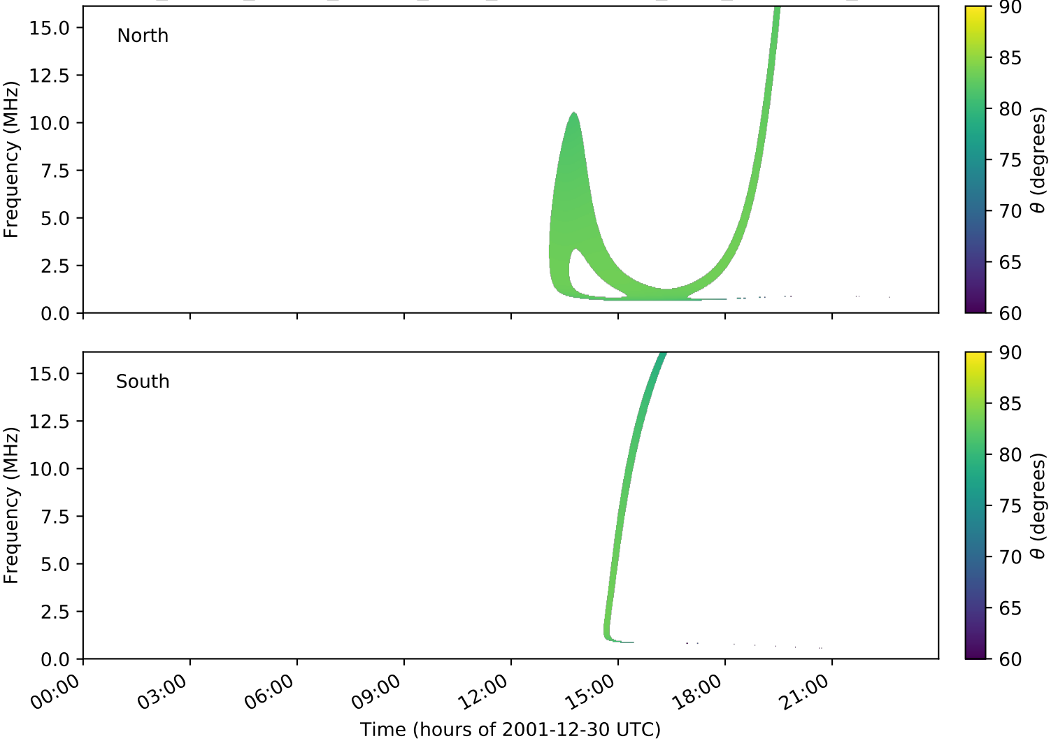
expres_cassini_jupiter_europa_isaac_lossc-wid1deg_3kev_20011230_v01.cdf
