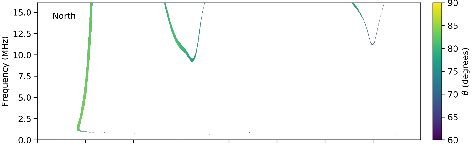
expres_cassini_jupiter_europa_isaac_lossc-wid1deg_3kev_20011227_v01.cdf
