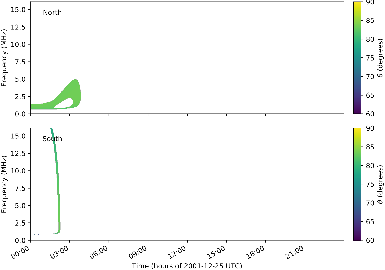
expres_cassini_jupiter_europa_isaac_lossc-wid1deg_3kev_20011225_v01.cdf
