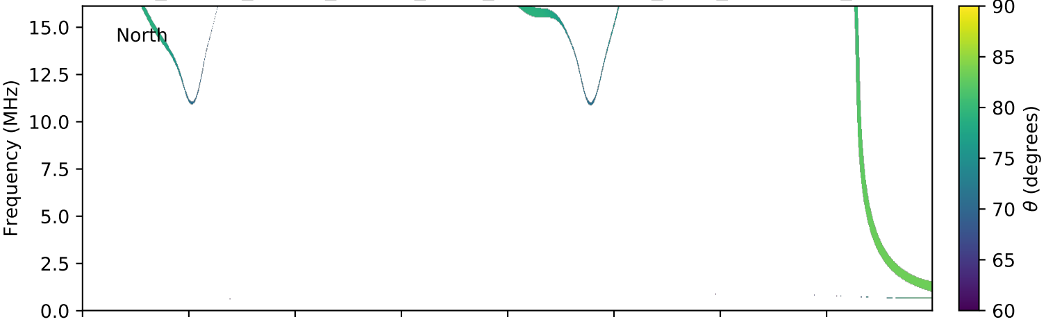
expres_cassini_jupiter_europa_isaac_lossc-wid1deg_3kev_20011224_v01.cdf
