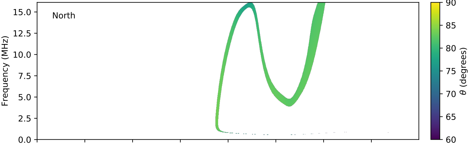
expres_cassini_jupiter_europa_isaac_lossc-wid1deg_3kev_20011223_v01.cdf
