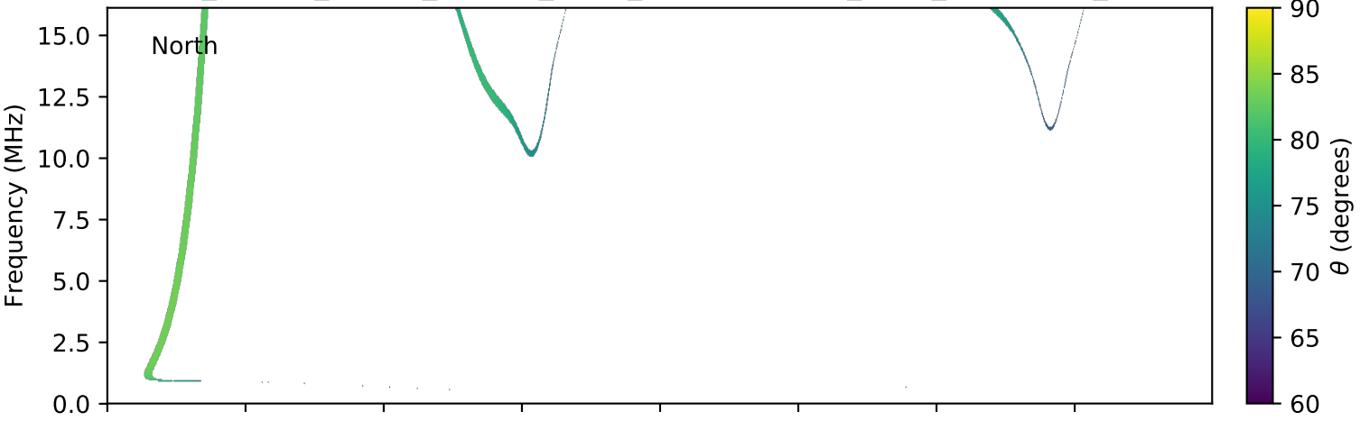
expres_cassini_jupiter_europa_isaac_lossc-wid1deg_3kev_20011220_v01.cdf
