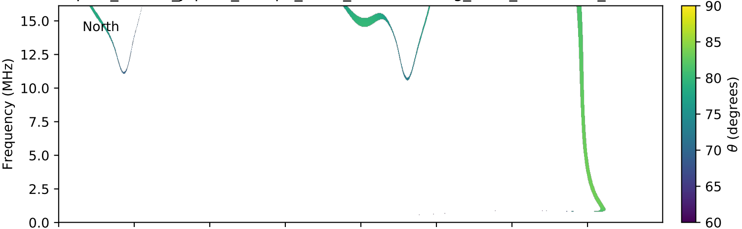
expres_cassini_jupiter_europa_isaac_lossc-wid1deg_3kev_20011217_v01.cdf
