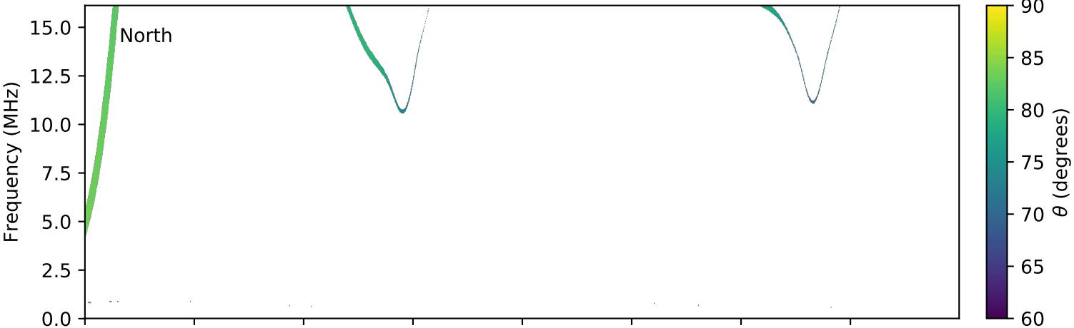
expres_cassini_jupiter_europa_isaac_lossc-wid1deg_3kev_20011213_v01.cdf
