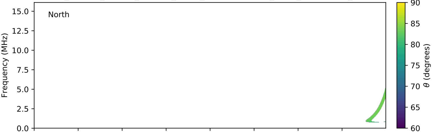
expres_cassini_jupiter_europa_isaac_lossc-wid1deg_3kev_20011212_v01.cdf
