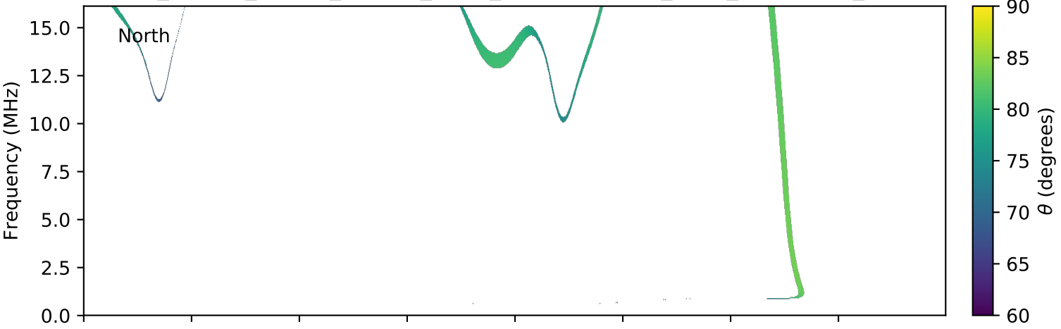
expres_cassini_jupiter_europa_isaac_lossc-wid1deg_3kev_20011210_v01.cdf
