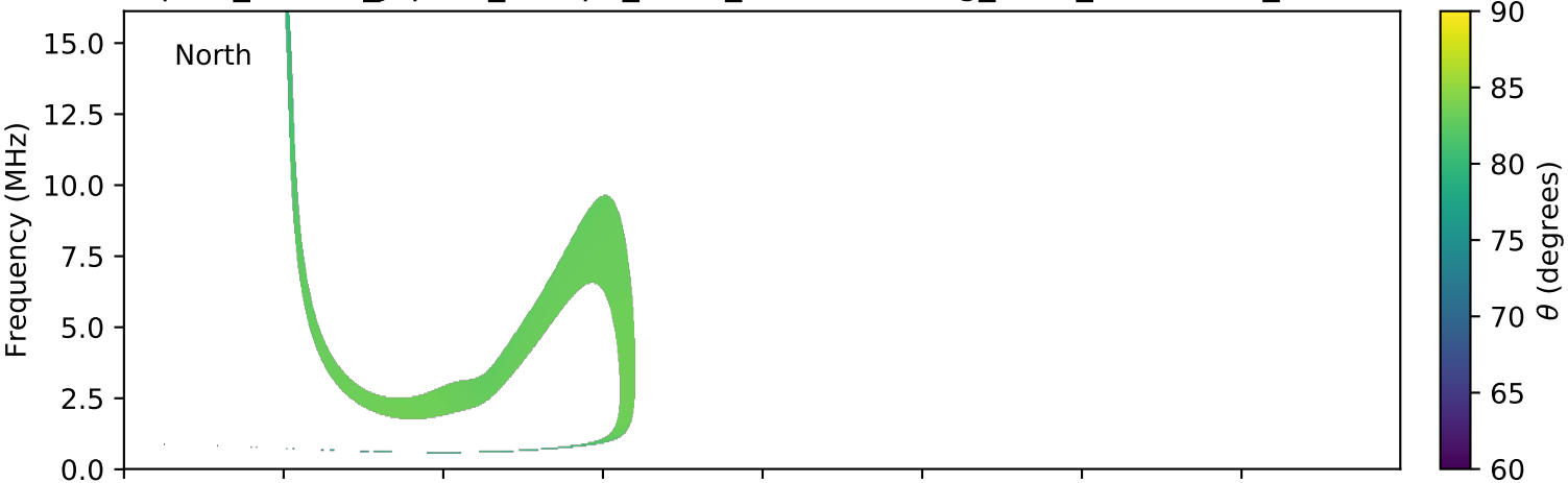
expres_cassini_jupiter_europa_isaac_lossc-wid1deg_3kev_20011207_v01.cdf
