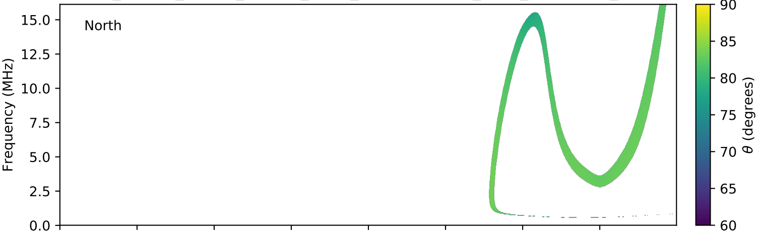
expres_cassini_jupiter_europa_isaac_lossc-wid1deg_3kev_20011205_v01.cdf
