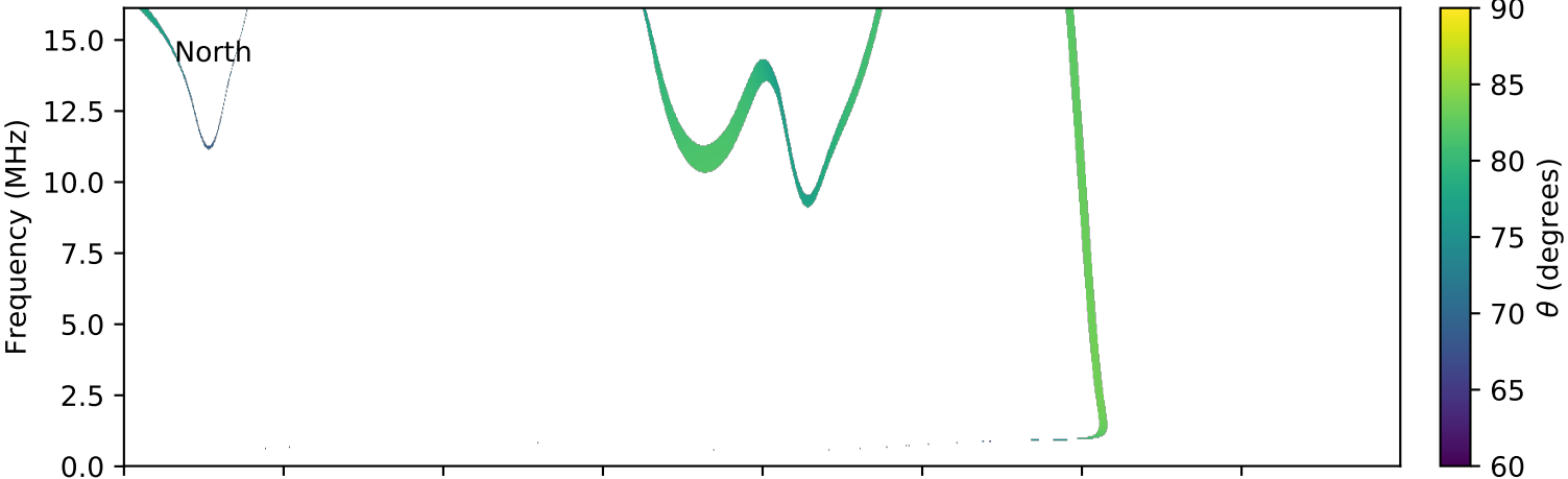
expres_cassini_jupiter_europa_isaac_lossc-wid1deg_3kev_20011203_v01.cdf
