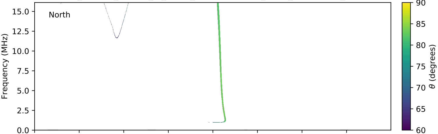
expres_cassini_jupiter_io_isaac_lossc-wid1deg_3kev_20011125_v01.cdf
