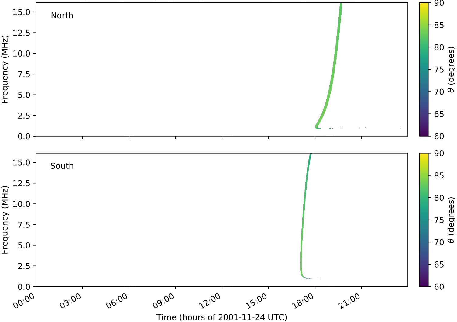
expres_cassini_jupiter_io_isaac_lossc-wid1deg_3kev_20011124_v01.cdf
