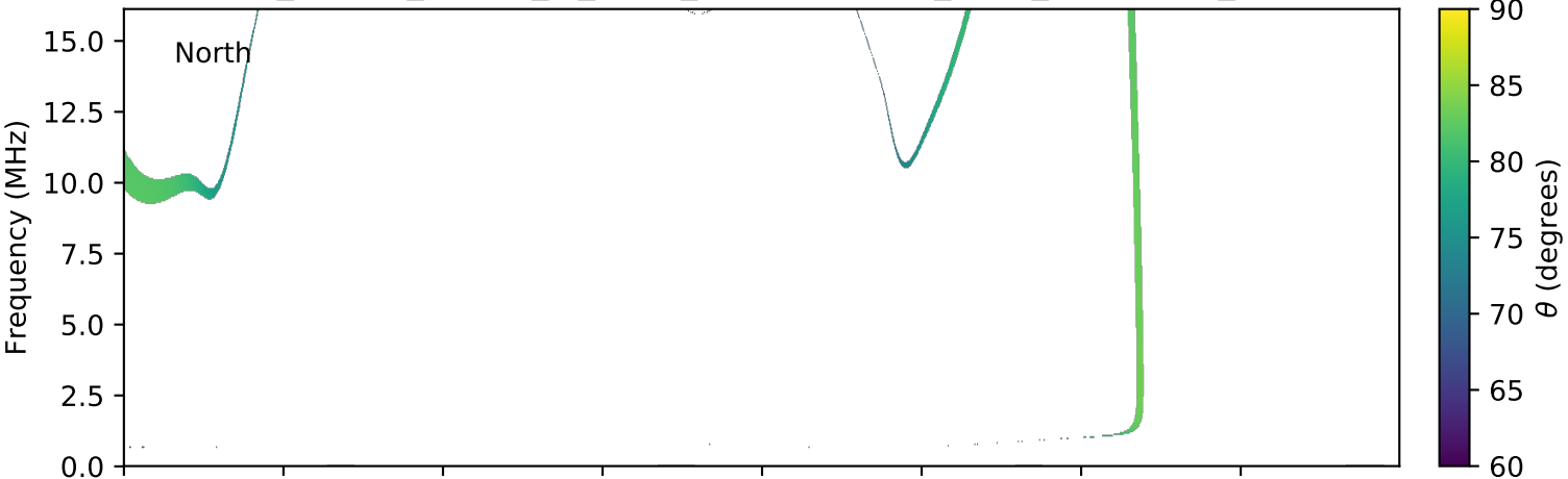
expres_cassini_jupiter_io_isaac_lossc-wid1deg_3kev_20011123_v01.cdf
