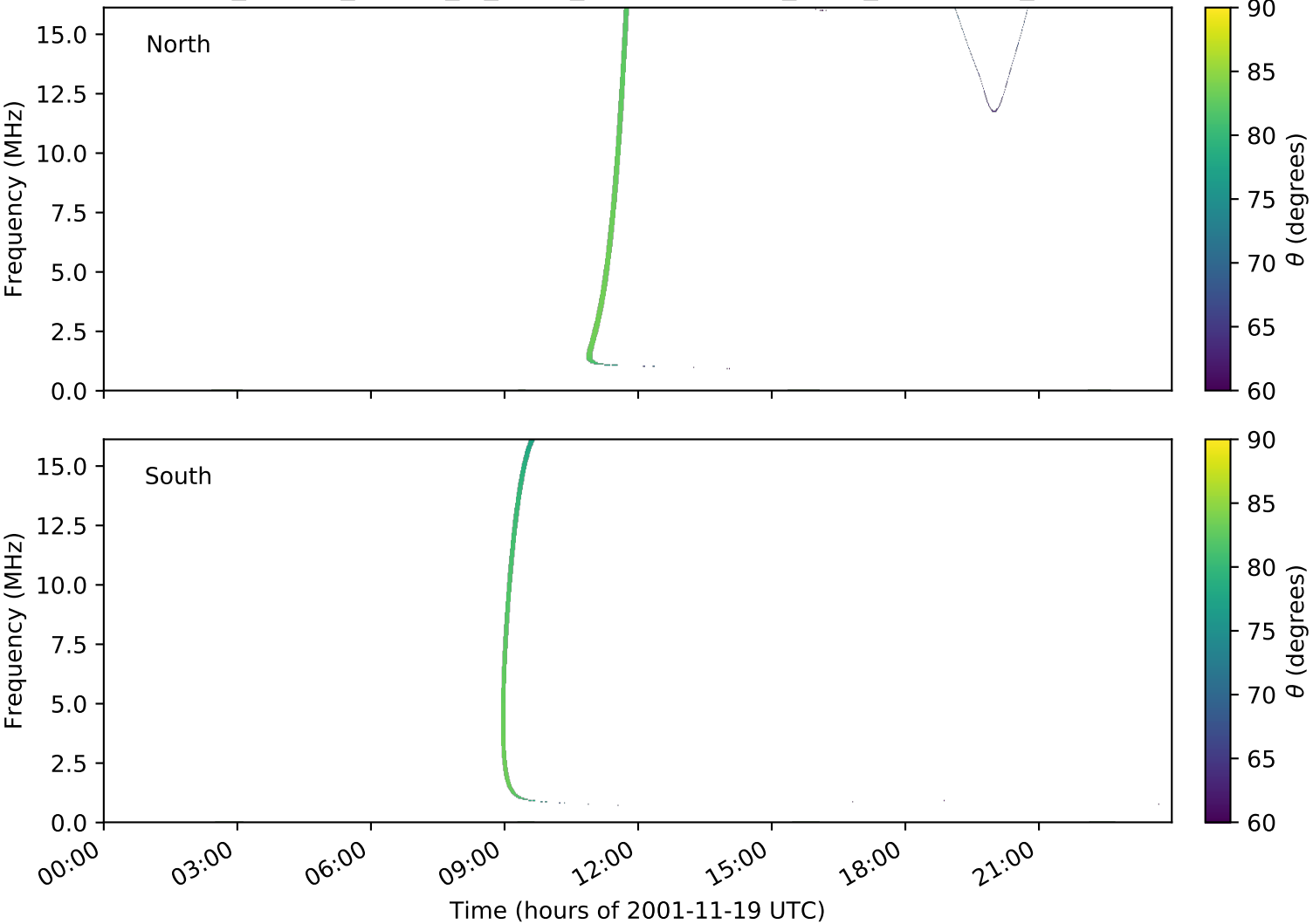
expres_cassini_jupiter_io_isaac_lossc-wid1deg_3kev_20011119_v01.cdf
