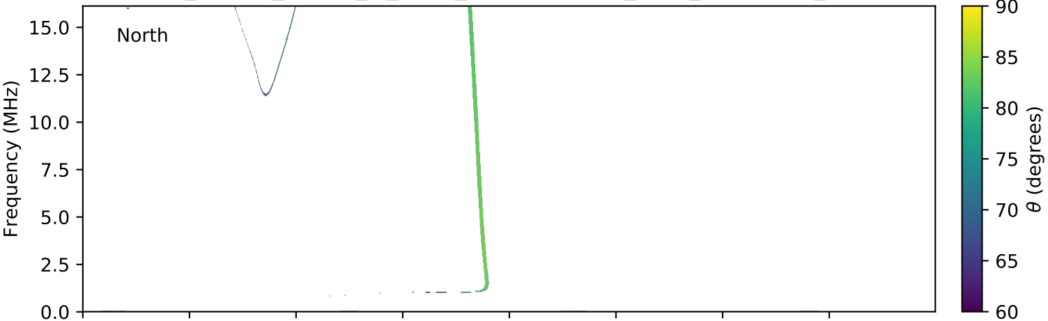
expres_cassini_jupiter_io_isaac_lossc-wid1deg_3kev_20011118_v01.cdf
