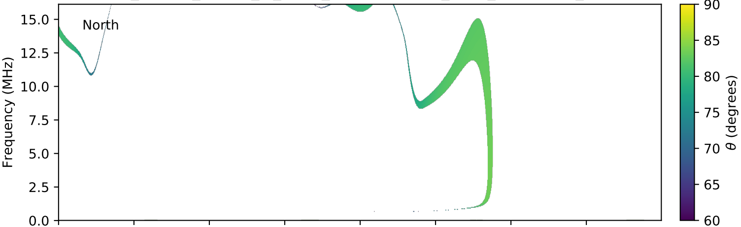
expres_cassini_jupiter_io_isaac_lossc-wid1deg_3kev_20011116_v01.cdf
