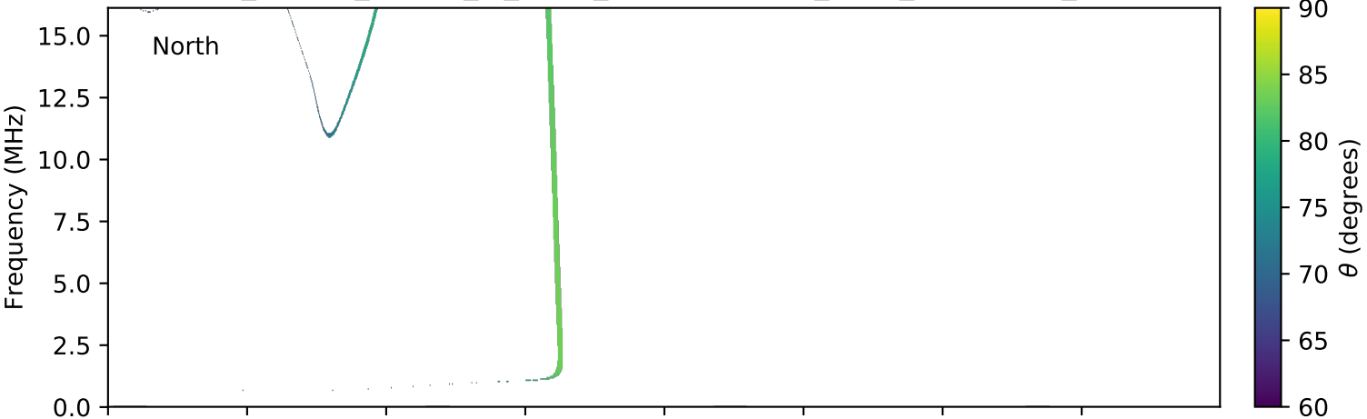
expres_cassini_jupiter_io_isaac_lossc-wid1deg_3kev_20011111_v01.cdf
