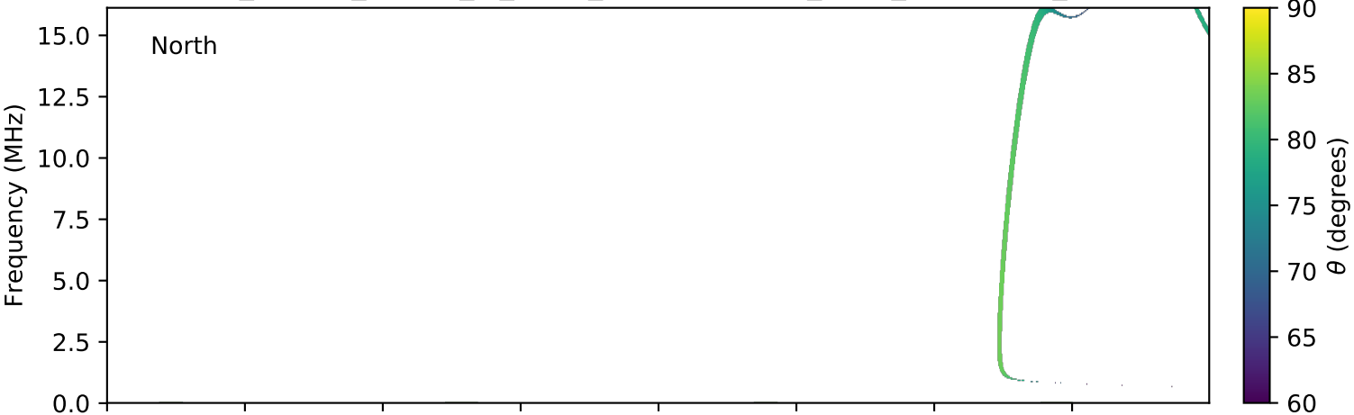
expres_cassini_jupiter_io_isaac_lossc-wid1deg_3kev_20011108_v01.cdf
