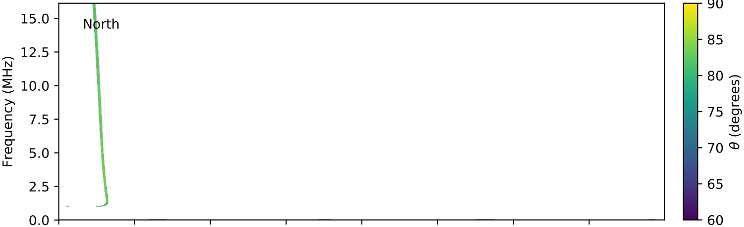
expres_cassini_jupiter_io_isaac_lossc-wid1deg_3kev_20011106_v01.cdf
