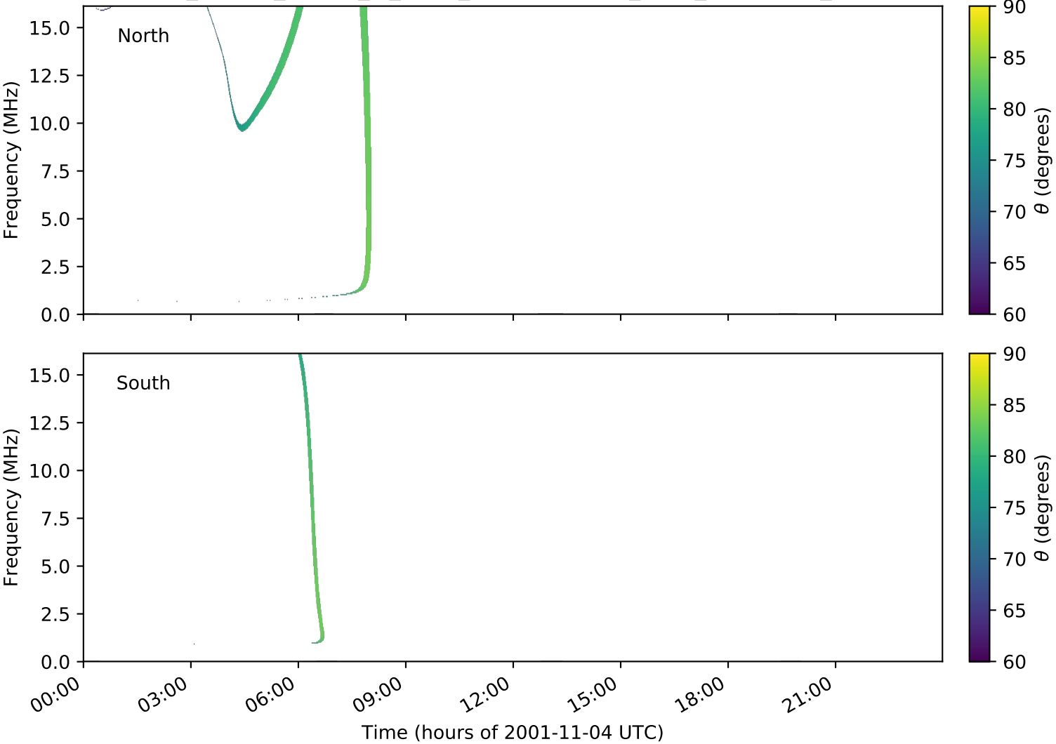
expres_cassini_jupiter_io_isaac_lossc-wid1deg_3kev_20011104_v01.cdf
