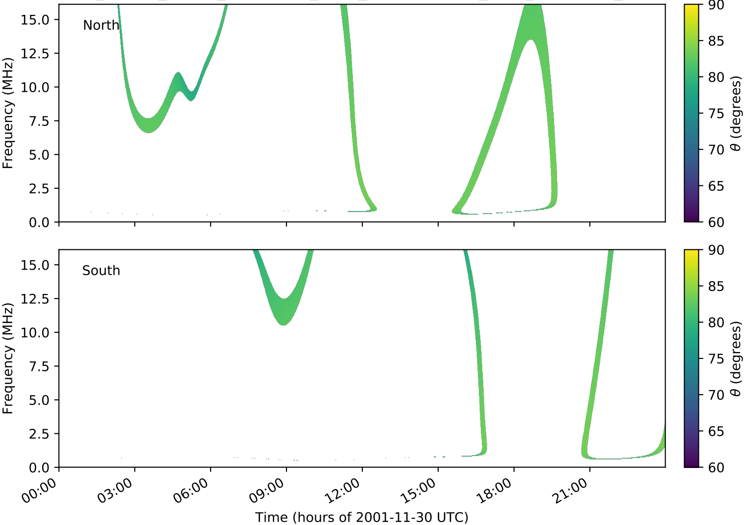
expres_cassini_jupiter_ganymede_isaac_lossc-wid1deg_3kev_20011130_v01.cdf
